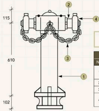
100mm PILLAR HYDRANT C/W OUTLET Model No. : 7625
