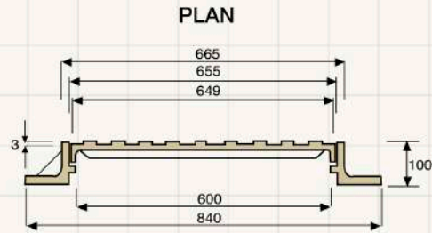
D.I. Manhole Cover & Frame (Model 670) Size : 840mm x 840mm x 100mm (H)
